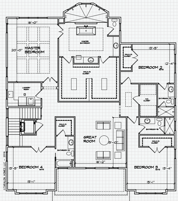
2nd Floor
