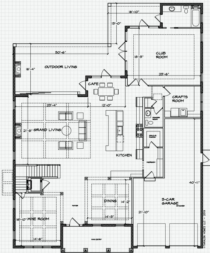
1st Floor
