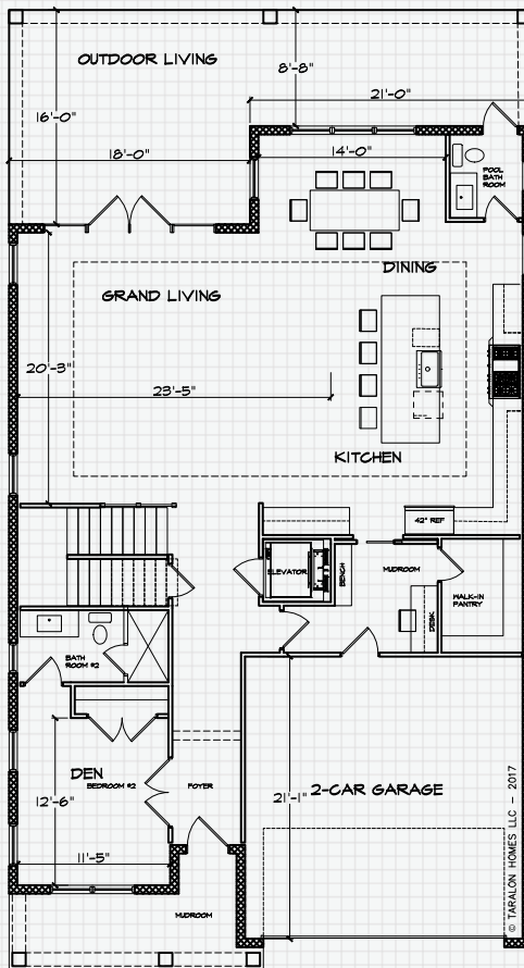
1st Floor
