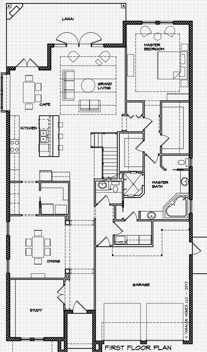
1st Floor
