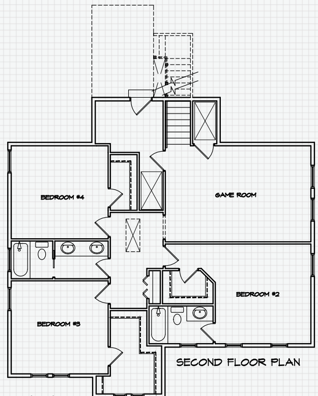
2nd Floor
