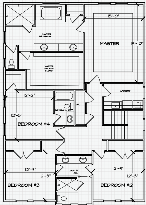
2nd Floor
