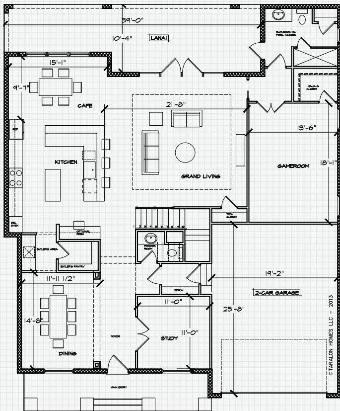
1st Floor
